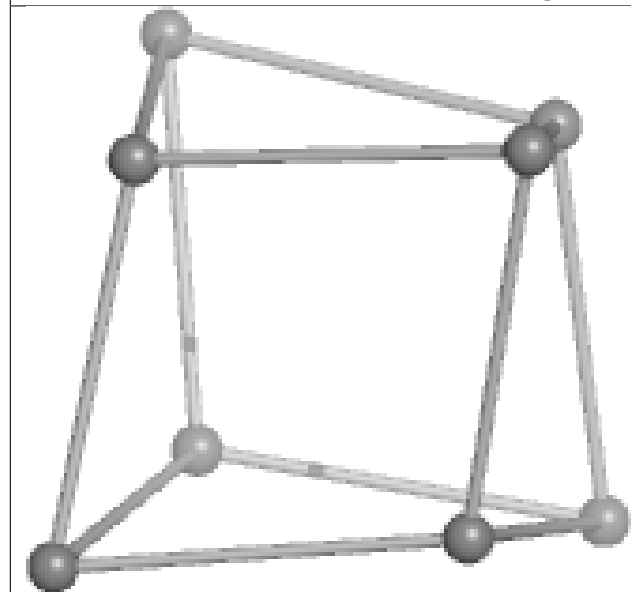
Bond lengths
