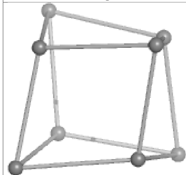
Torsions
