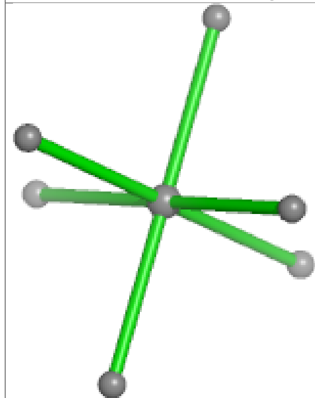
Bond lengths
