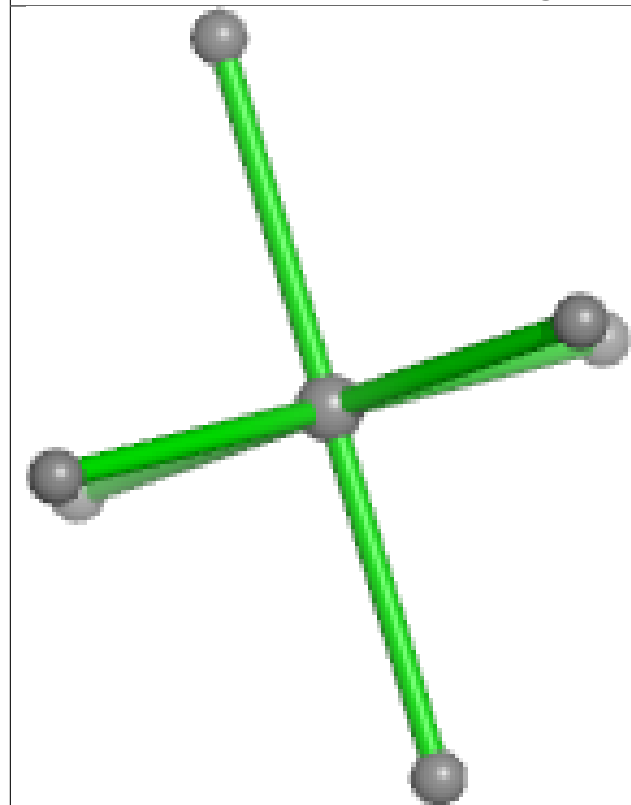
Bond lengths
