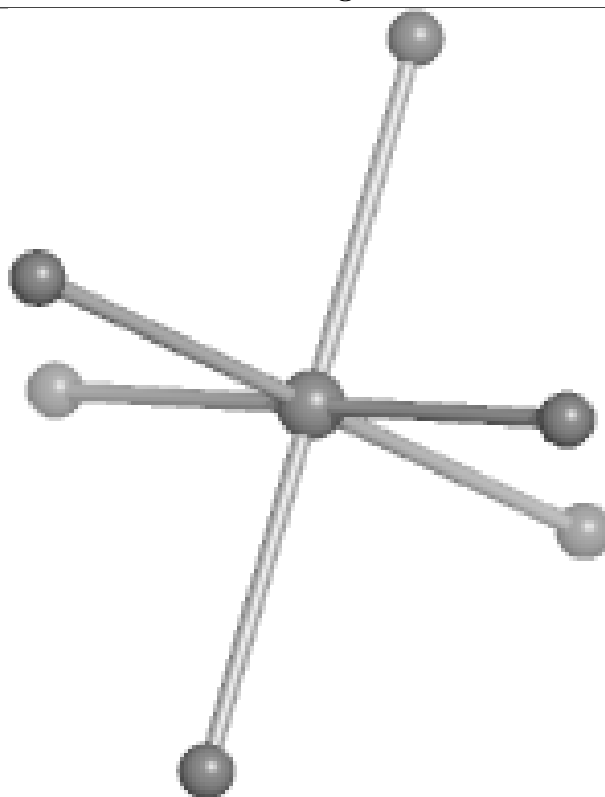
Rings
