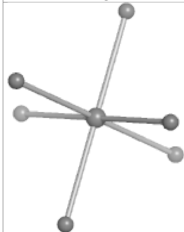
Torsions
