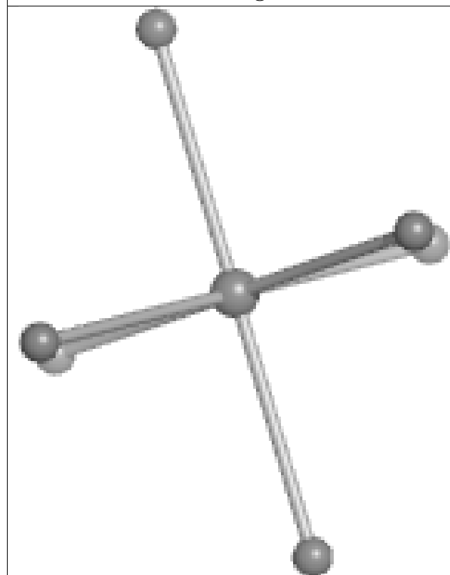
Torsions
